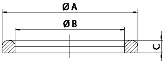
Gaskets dimensions
