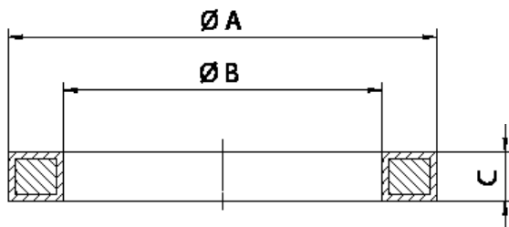
Gaskets dimensions
